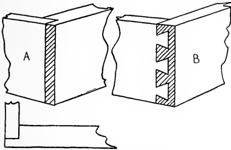
FIG. 430. A, COMMON METHOD. B, HALF-BLIND DOVETAIL.
